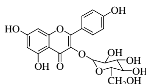
Kaempferol-3-O-D-glucoside (3)
